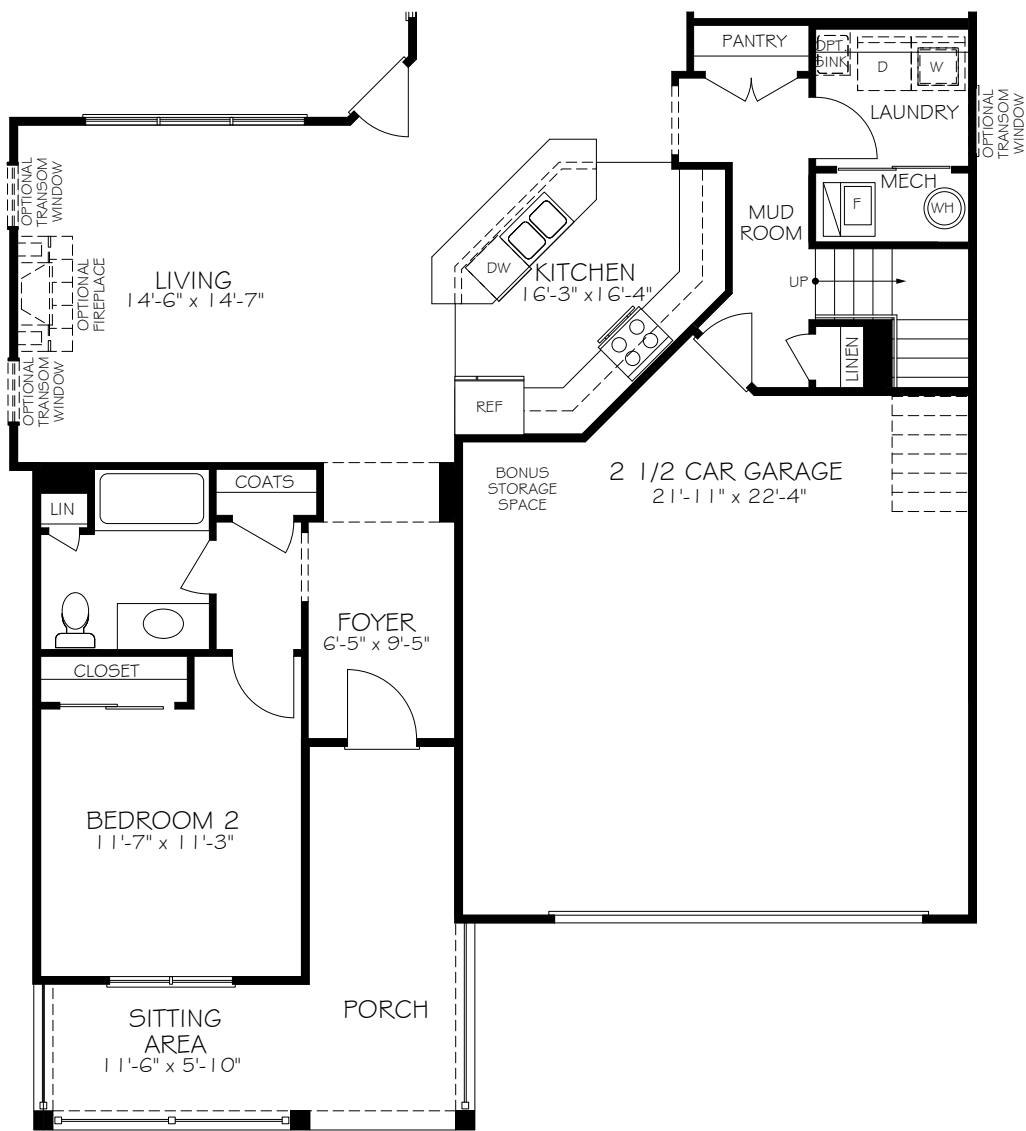
FIRST FLOOR PLAN W/ BONUS SUITE
