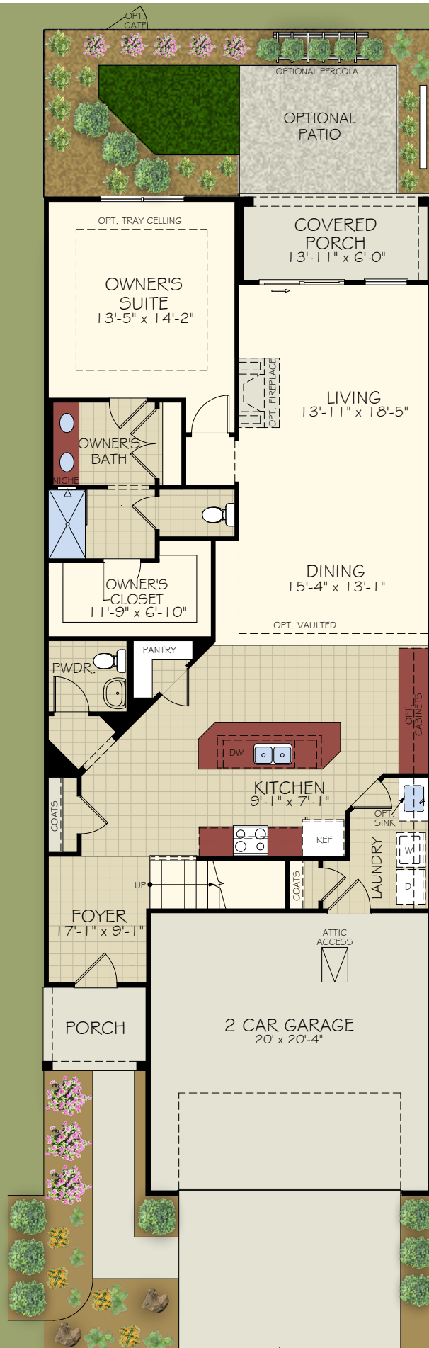
FIRST FLOOR
