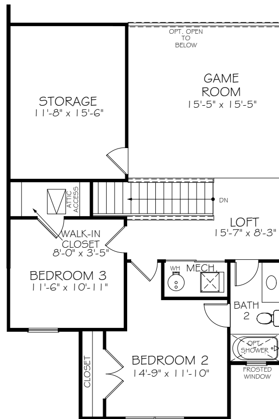
OPT. SECOND FLOOR - 2 BEDROOM/ GAME ROOM/1 BATH ( OPT. B )
