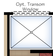
OPTIONAL UNIVERSAL SHOWER LAYOUT WITH ZERO THRESHOLD
