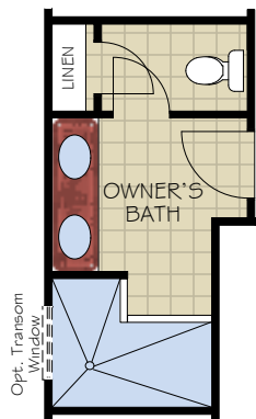
OPT. L-SHAPED SHOWER LAYOUT WITH ZERO THRESHOLD
