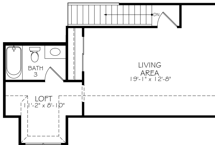
SECOND FLOOR PLAN WITH OPTIONAL BONUS SUITE ELEVATION A
