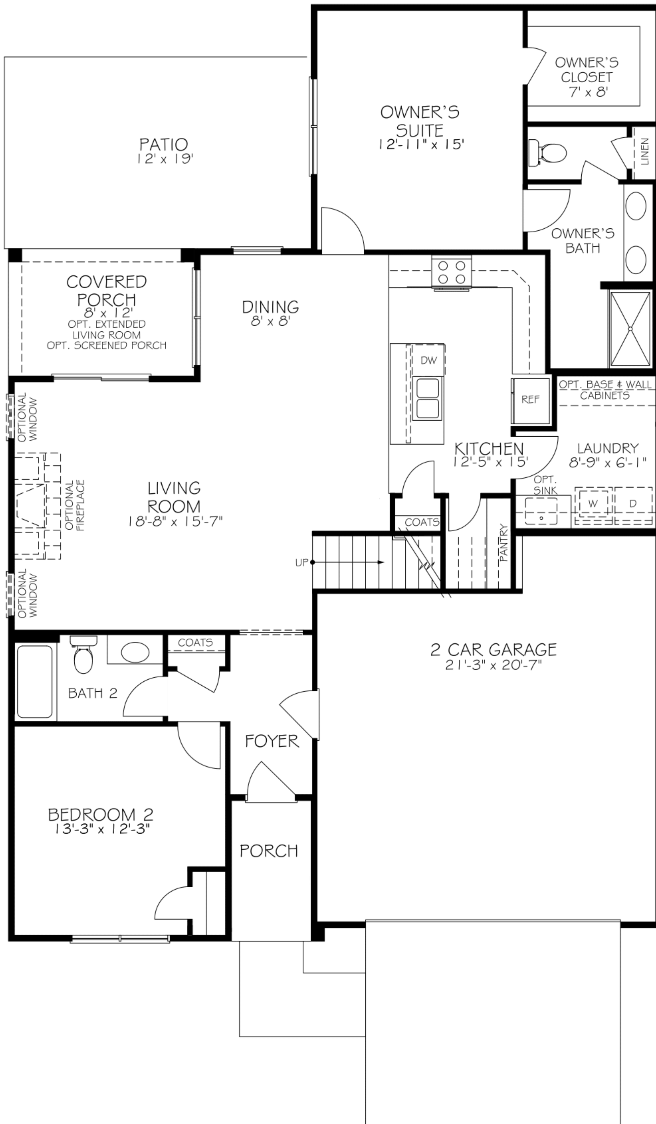
FIRST FLOOR
