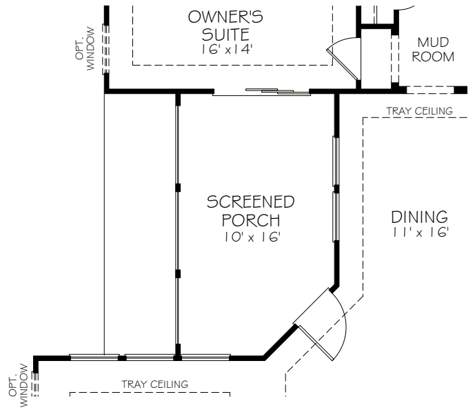
OPT. COURTYARD SCREENED PORCH
