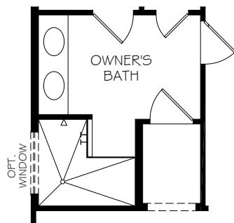
OPT. L-SHAPED SHOWER LAYOUT WITH ZERO THRESHOLD
