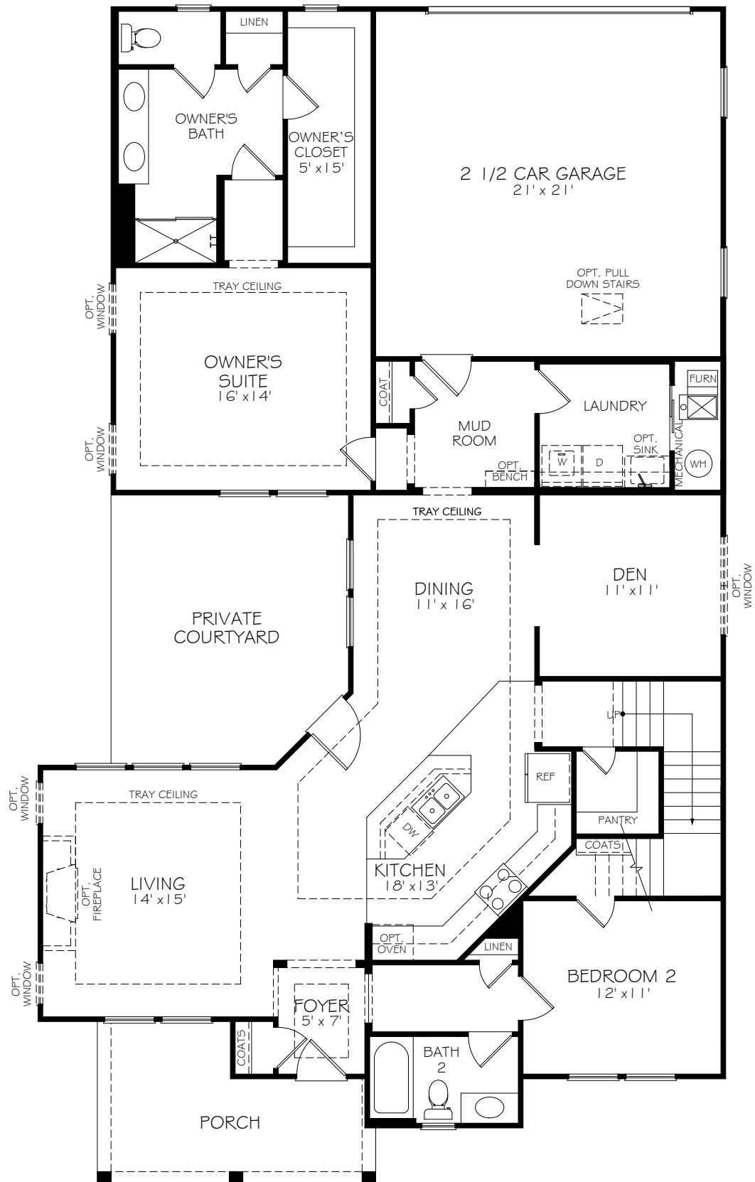
FIRST FLOOR PLAN W/ BONUS SUITE
