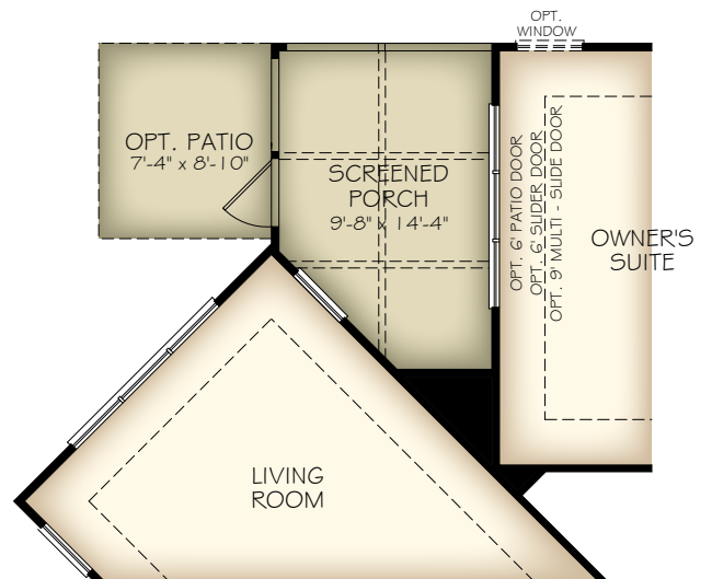
OPTIONAL PATIO OFF OWNERS SUITE SCREENED PORCH
