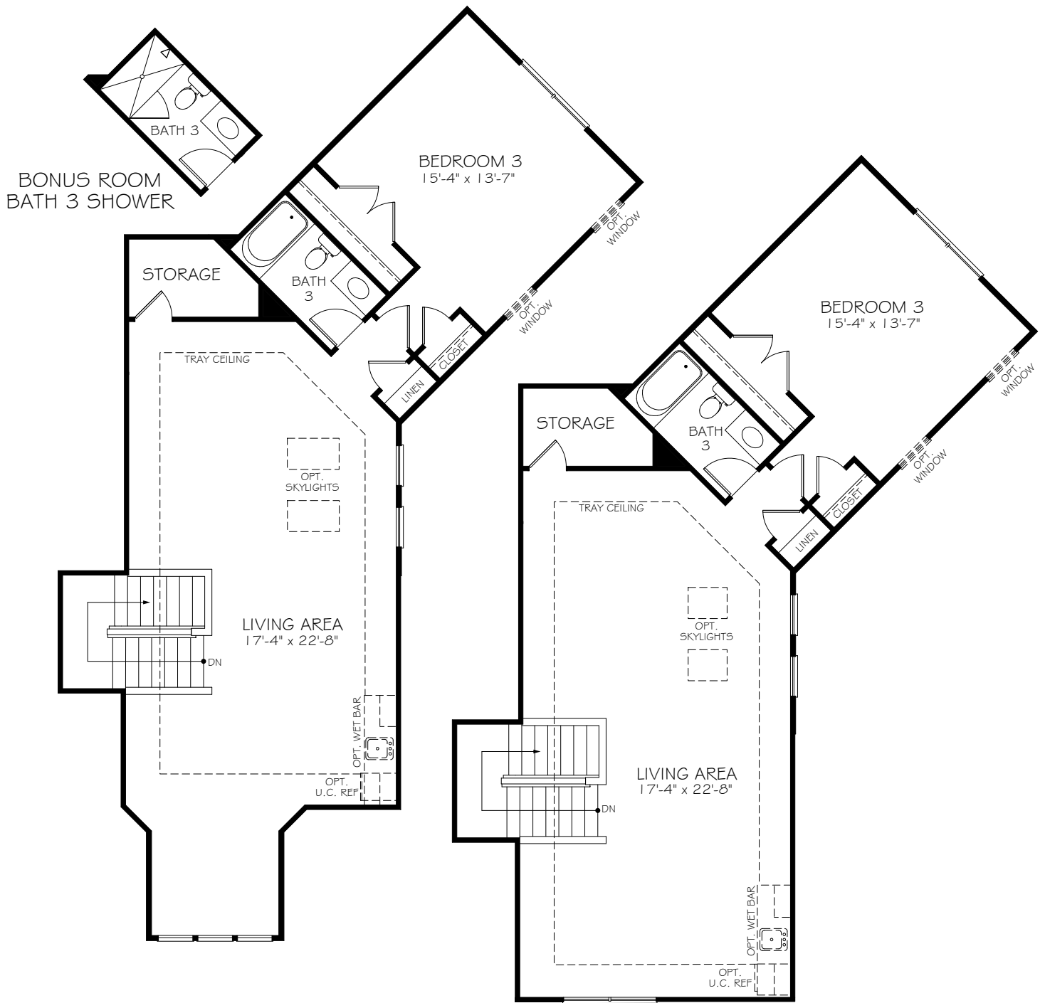
I 2ND FLOOR PLAN ELEVATION A
