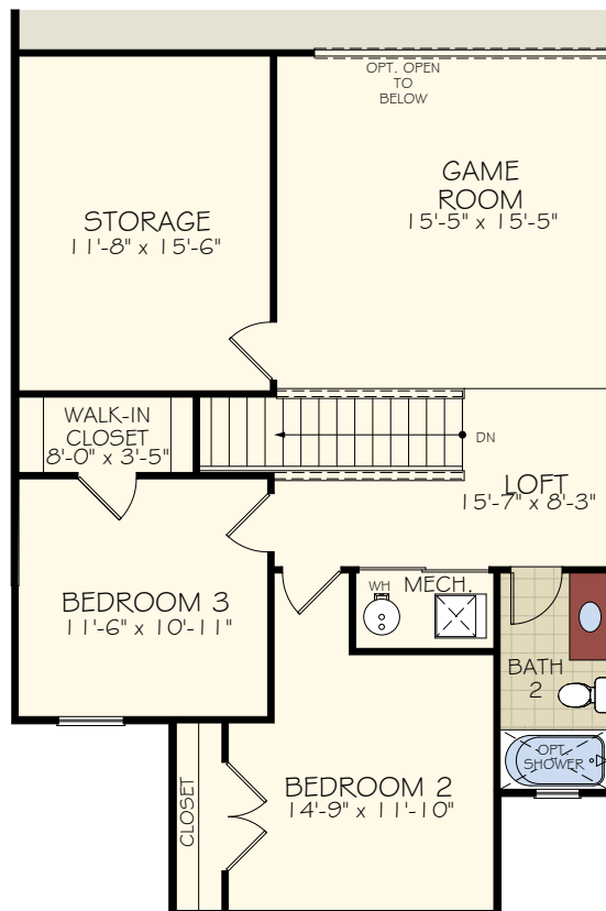
OPT. SECOND FLOOR - 2 BEDROOM/ GAME ROOM/1 BATH
