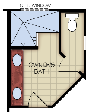
OPTIONAL L-SHAPED SHOWER LAYOUT WITH ZERO THRESHOLD
