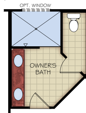
OPTIONAL UNIVERSAL SHOWER LAYOUT WITH ZERO THRESHOLD
