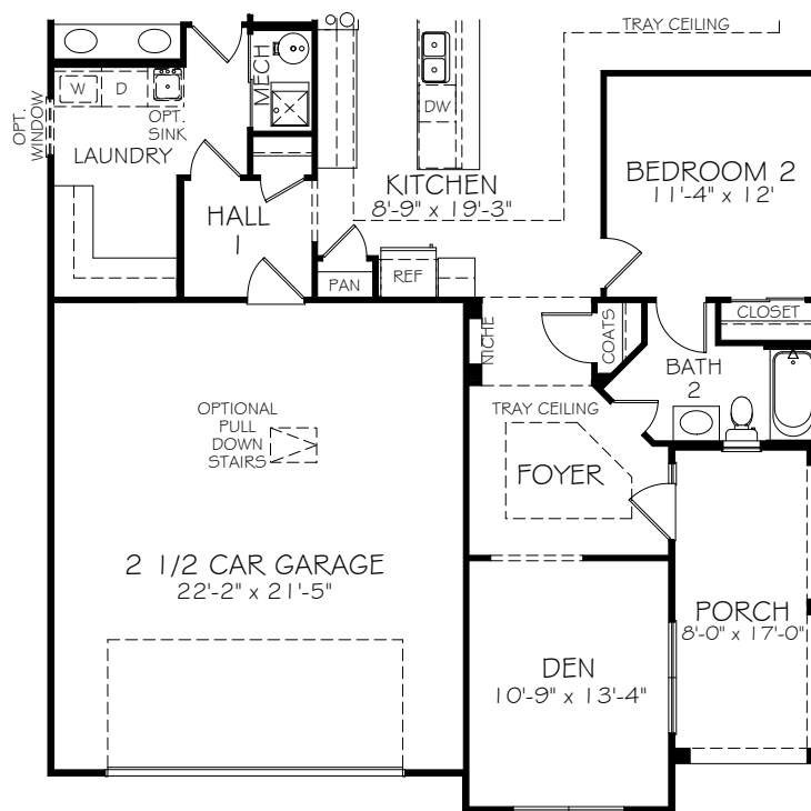
FIRST FLOOR PLAN EXPANDED LAUNDRY – RANCH PLAN
