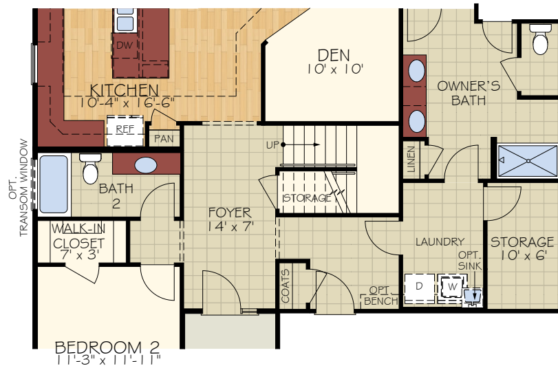
FIRST FLOOR PLAN W/ BONUS SUITE
