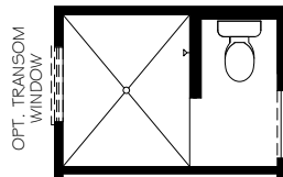
OPTIONAL UNIVERSAL SHOWER LAYOUT ZERO THRESHOLD
