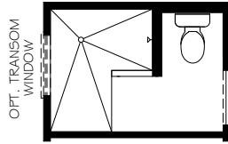
OPTIONAL L-SHAPED SHOWER LAYOUT WITH ZERO THRESHOLD
