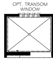
OPTIONAL UNIVERSAL SHOWER LAYOUT ZERO THRESHOLD
