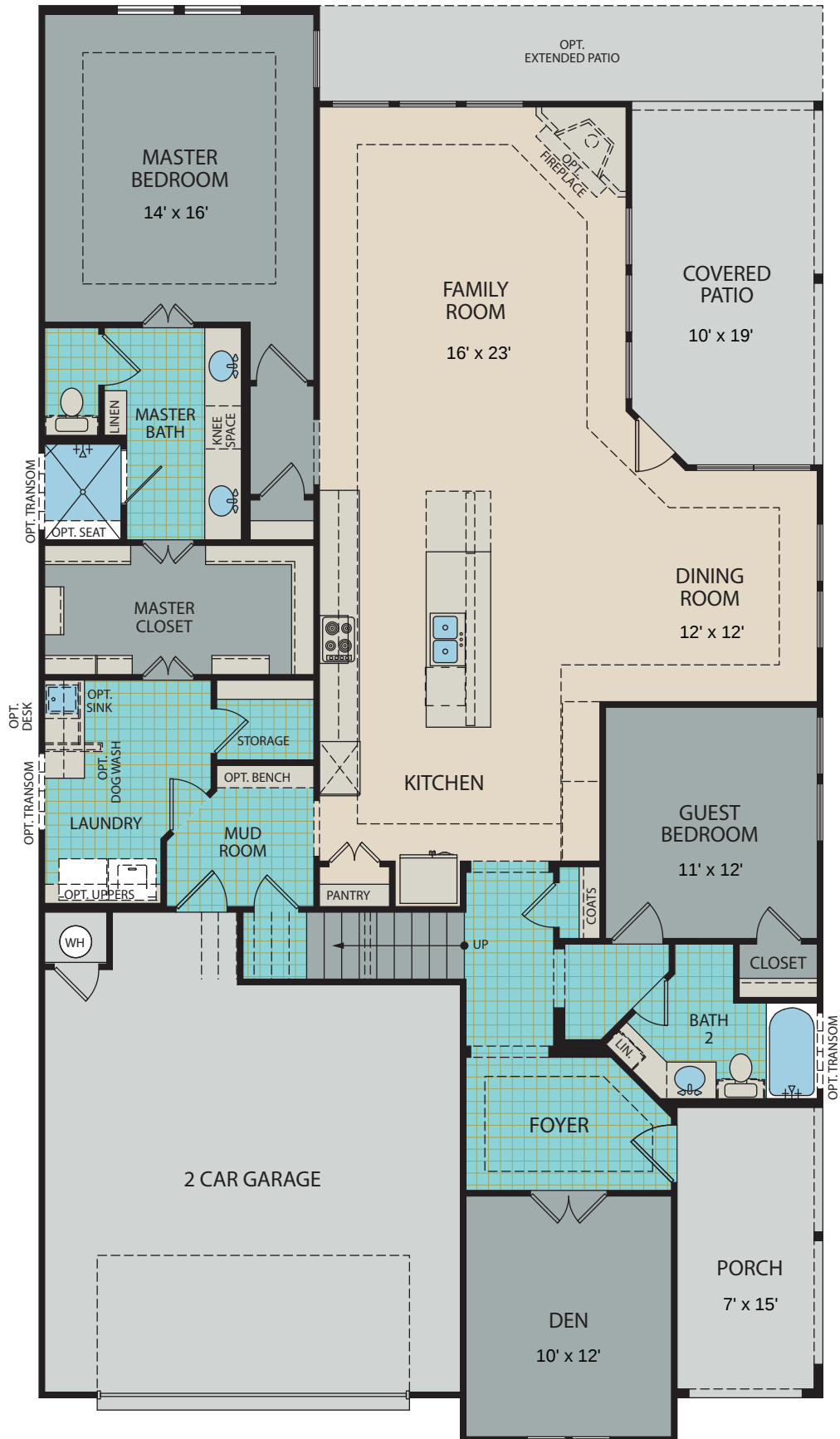
First Floor
