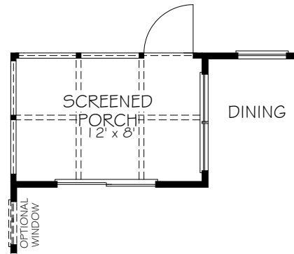
OPT. SCREENED PORCH ILO COVERED PORCH
