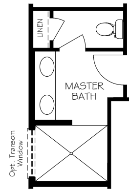
OPT. UNIVERSAL SHOWER LAYOUT WITH ZERO THRESHOLD
