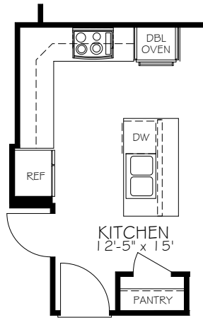
OPT. DELUXE KITCHEN
