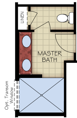
OPT. UNIVERSAL SHOWER LAYOUT WITH ZERO THRESHOLD
