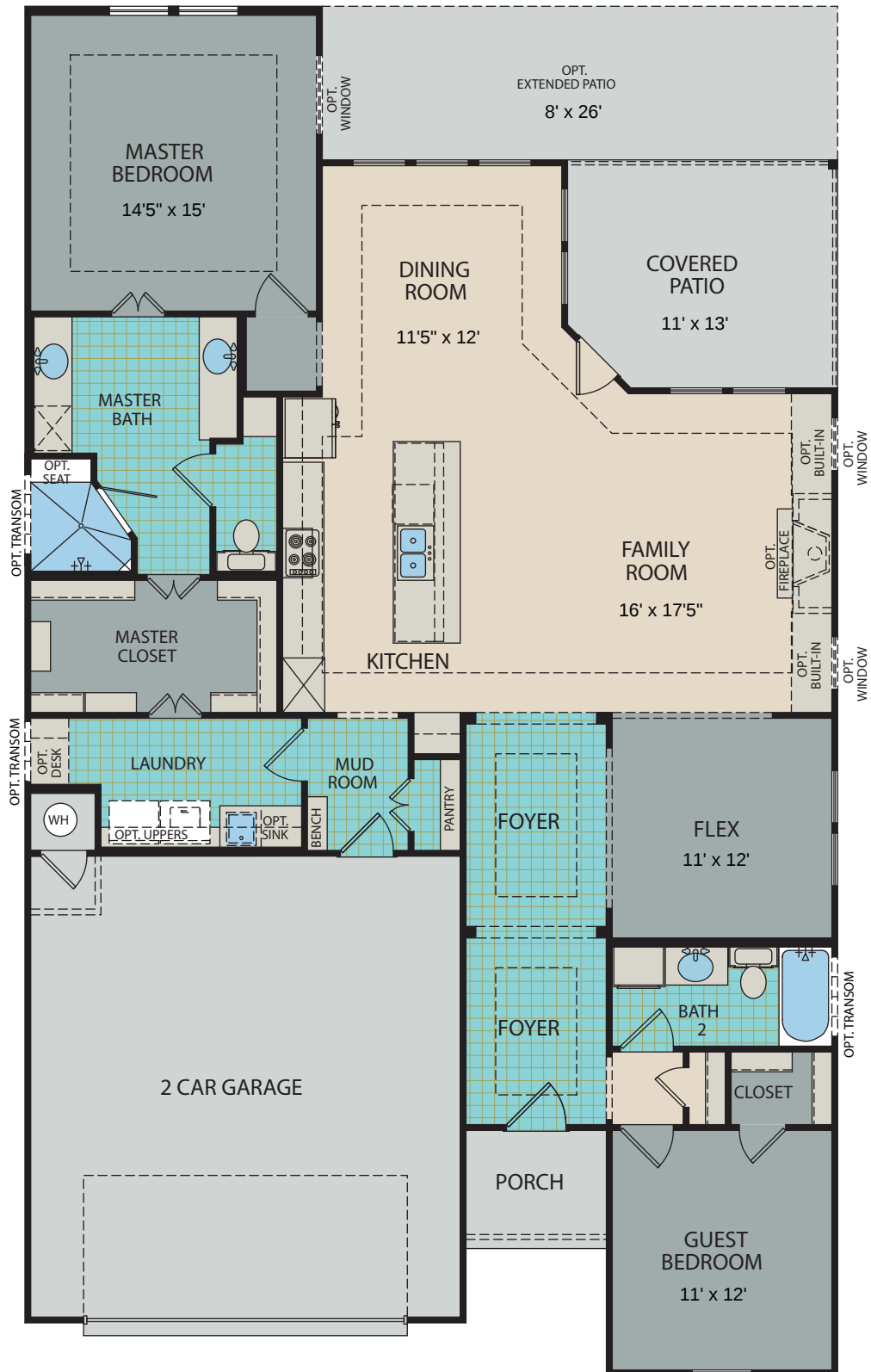
Floor Plan
