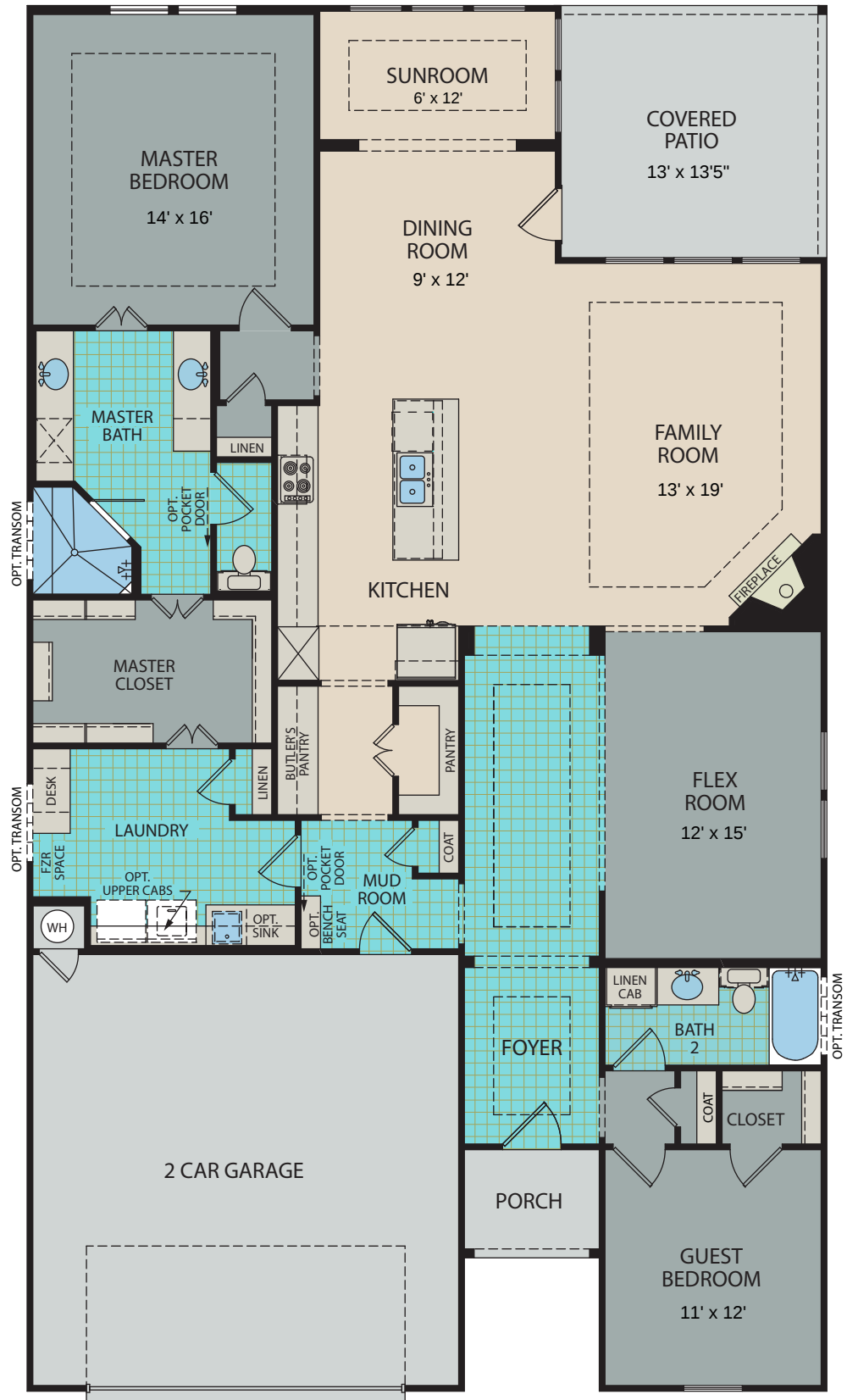
Floor Plan
