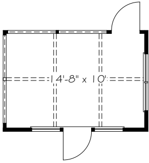
OPTIONAL LIVING SCREENED PORCH
