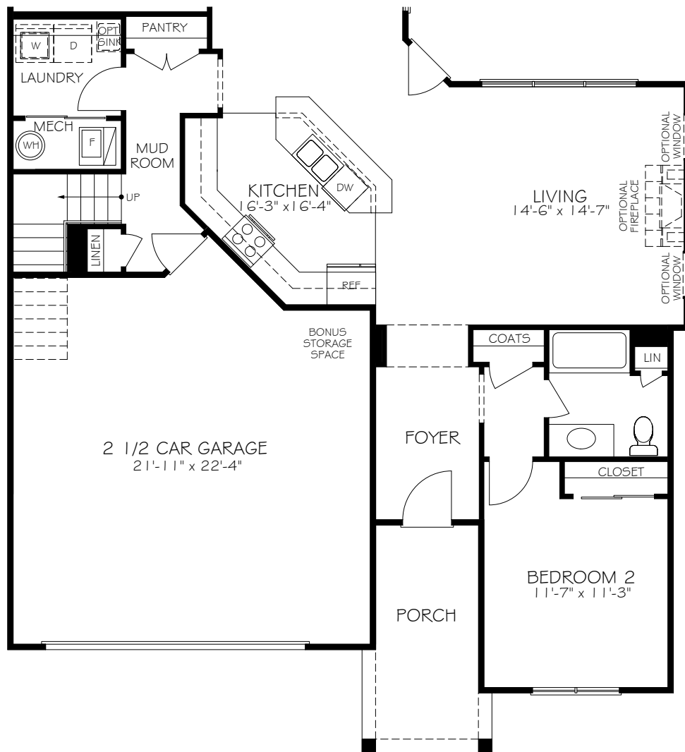
FIRST FLOOR PLAN W/ OPTIONAL BONUS SUITE
