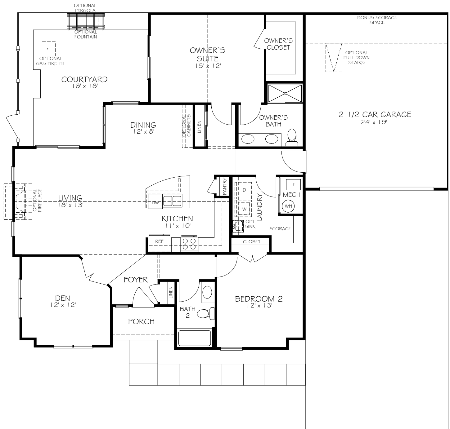
FLOOR PLAN
