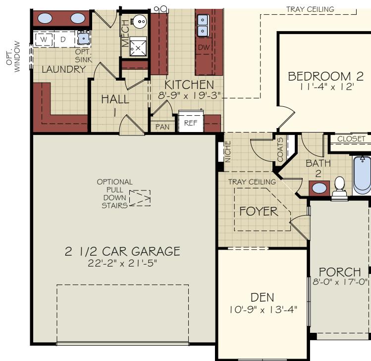
FIRST FLOOR PLAN EXPANDED LAUNDRY – RANCH PLAN
