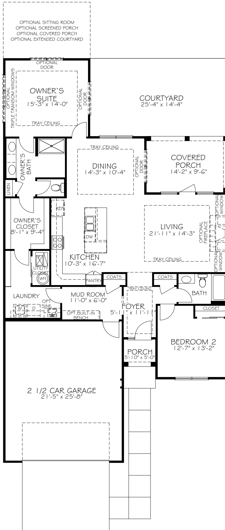
FIRST FLOOR
