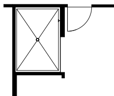
OPTIONAL UNIVERSAL SHOWER LAYOUT WITH ZERO THRESHOLD
