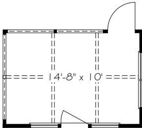
OPTIONAL LIVING SCREENED PORCH
