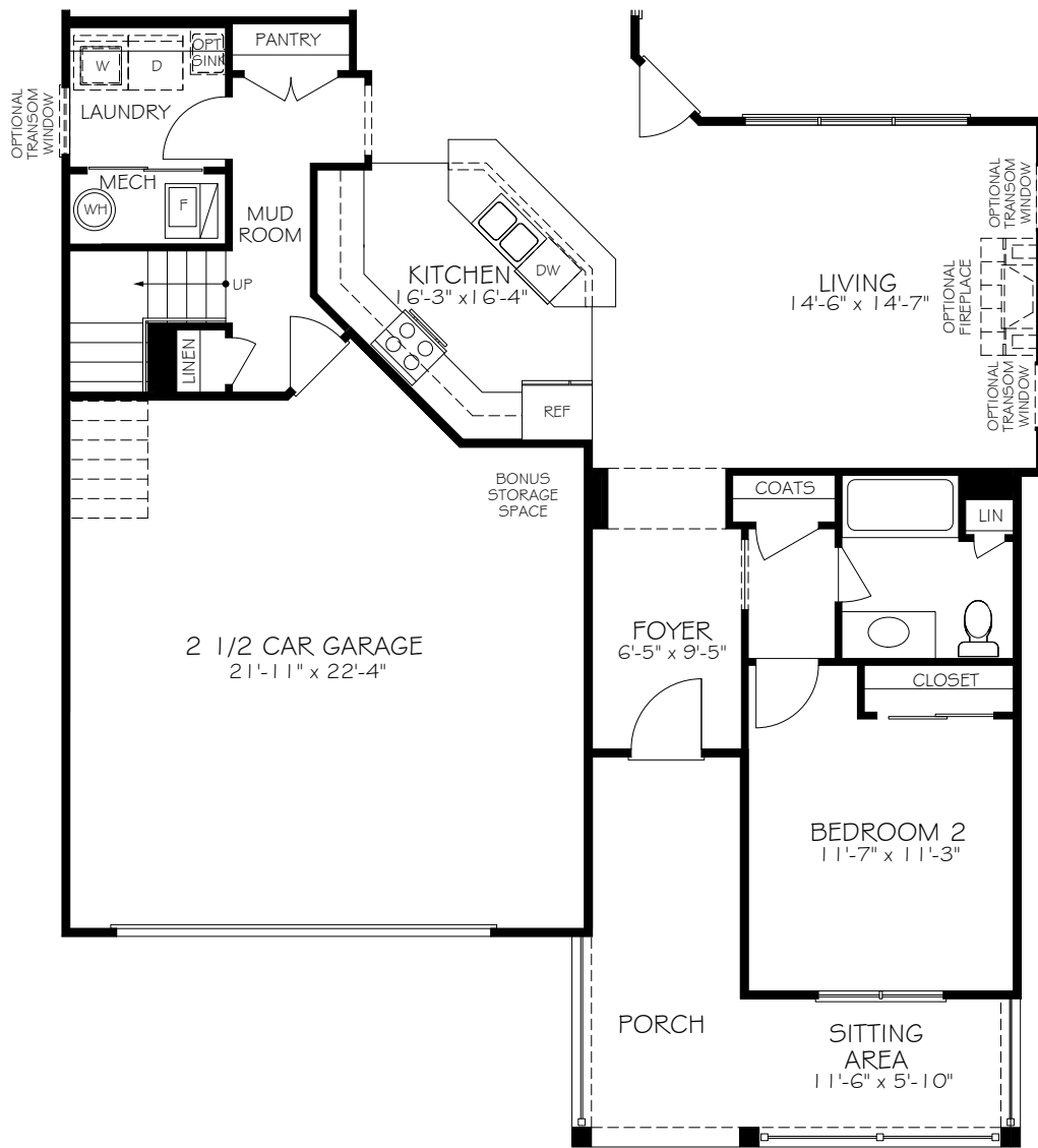
FIRST FLOOR PLAN W/ BONUS SUITE
