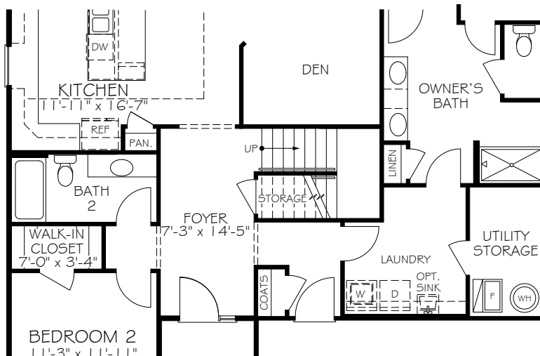
FIRST FLOOR PLAN WITH OPTIONAL BONUS SUITE
