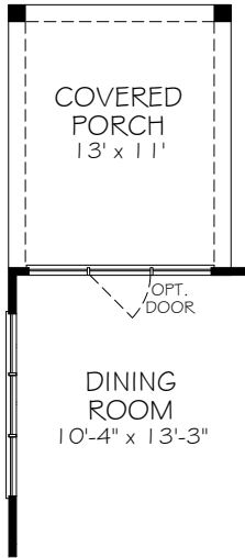
OPTIONAL COVERED PORCH (OFF DINING ROOM)
