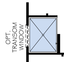
OPTIONAL UNIVERSAL SHOWER LAYOUT WITH ZERO THRESHOLD
