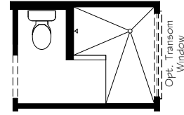
OPTIONAL L-SHAPED SHOWER LAYOUT WITH ZERO THRESHOLD
